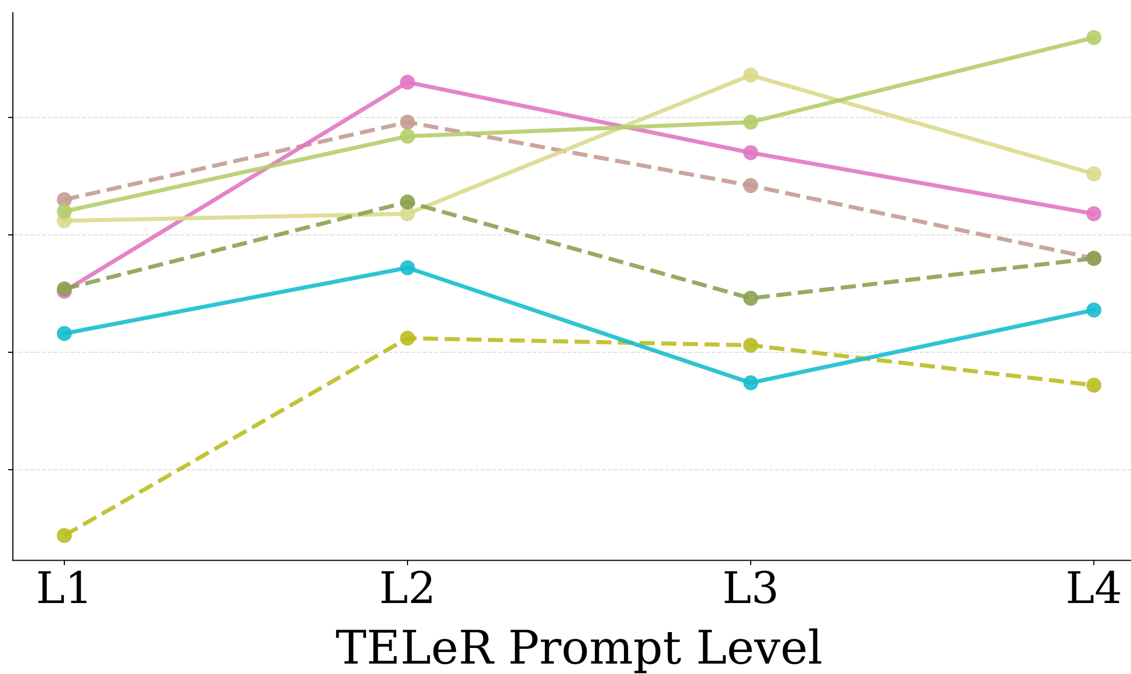
Medium (3B--8B)
